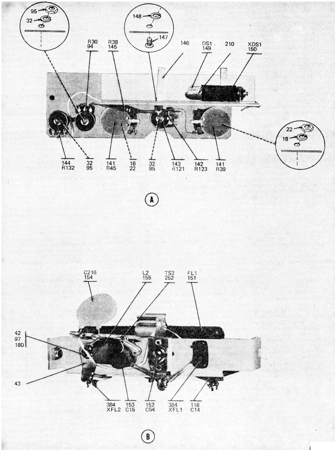
Figure 2 Chassis Subassembly (Sheet 7 of 20)
