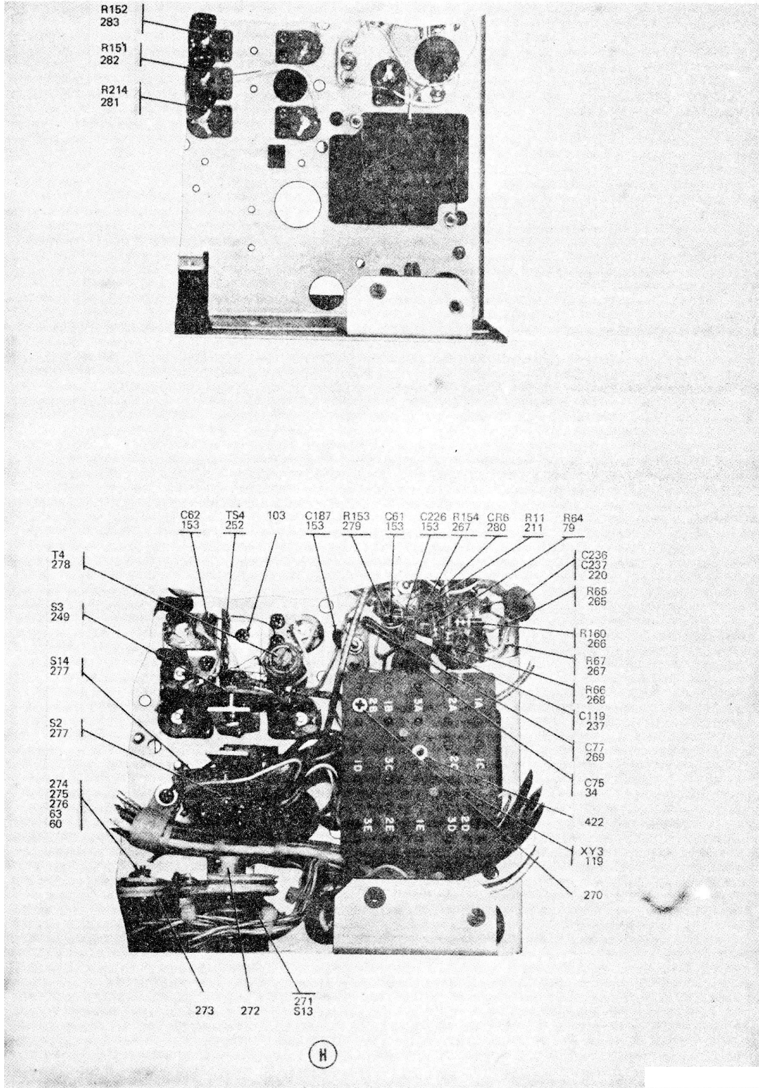
Figure 2. (13) Chassis subassembly (Sheet 13 of 20).
