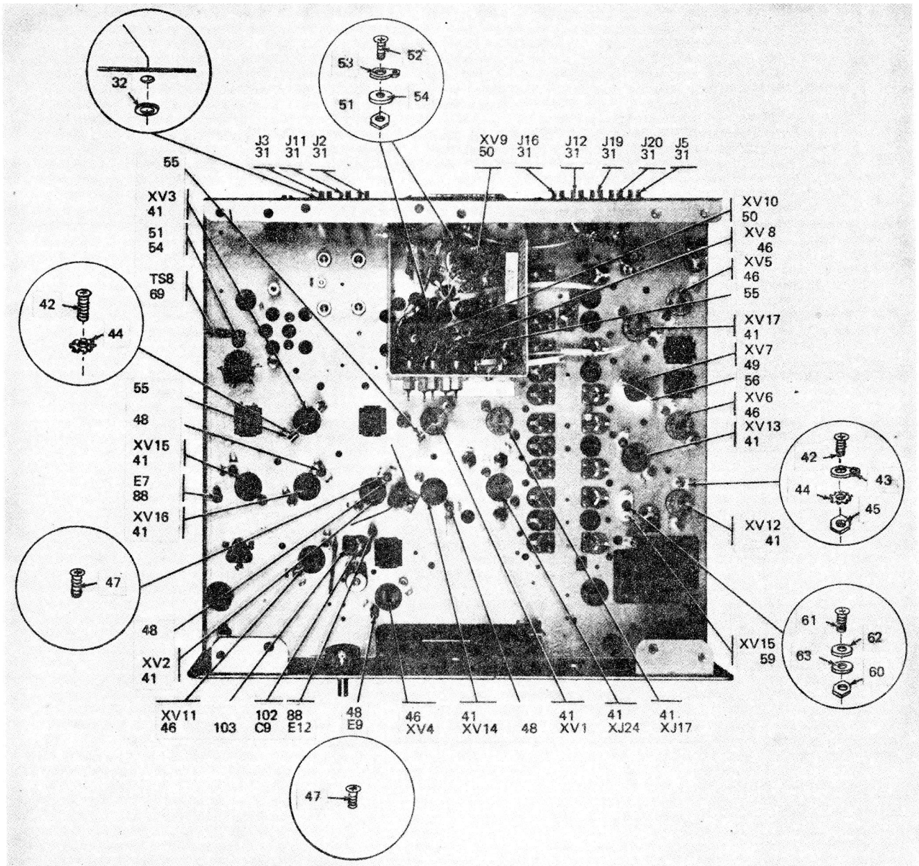
Figure 2. ③ Chassis subassembly (Sheet 3 of 20)
