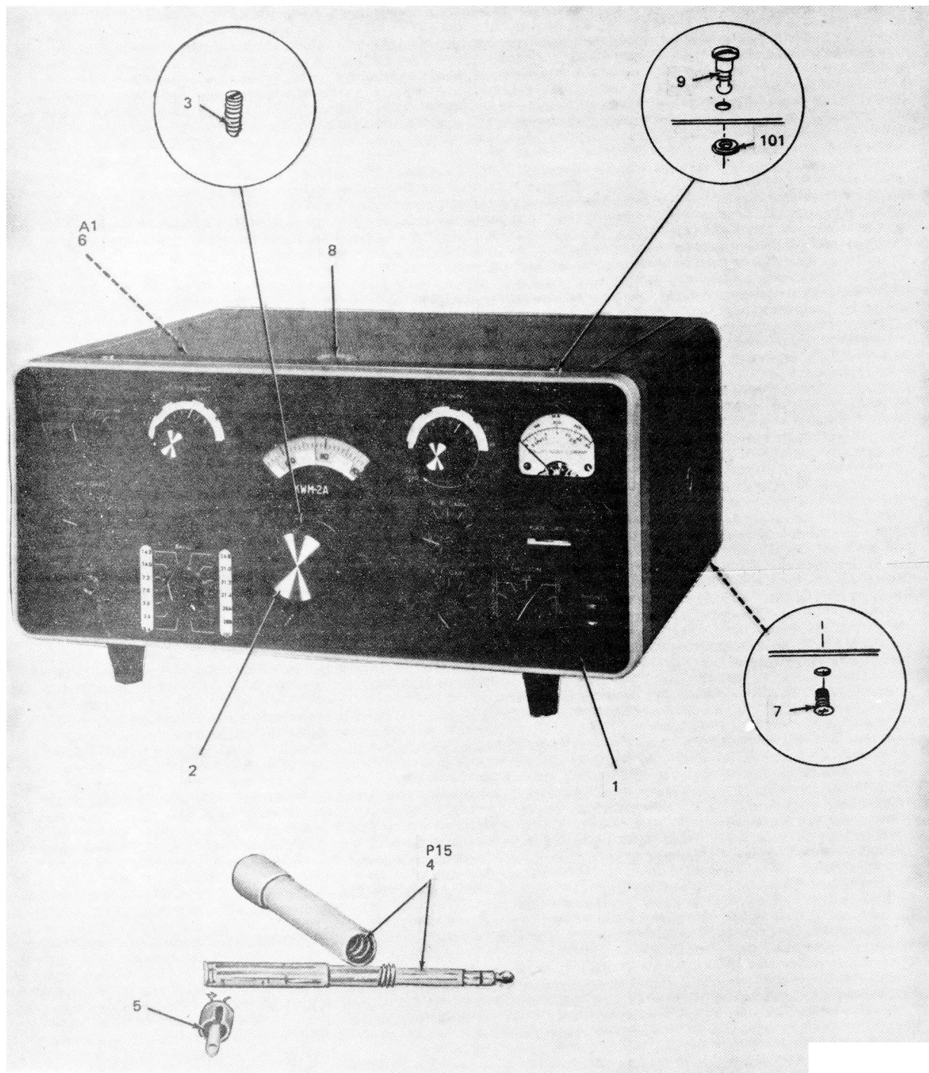
Figure 1. Receiver-Transmitter, Radio RT-718/FRC-93.
