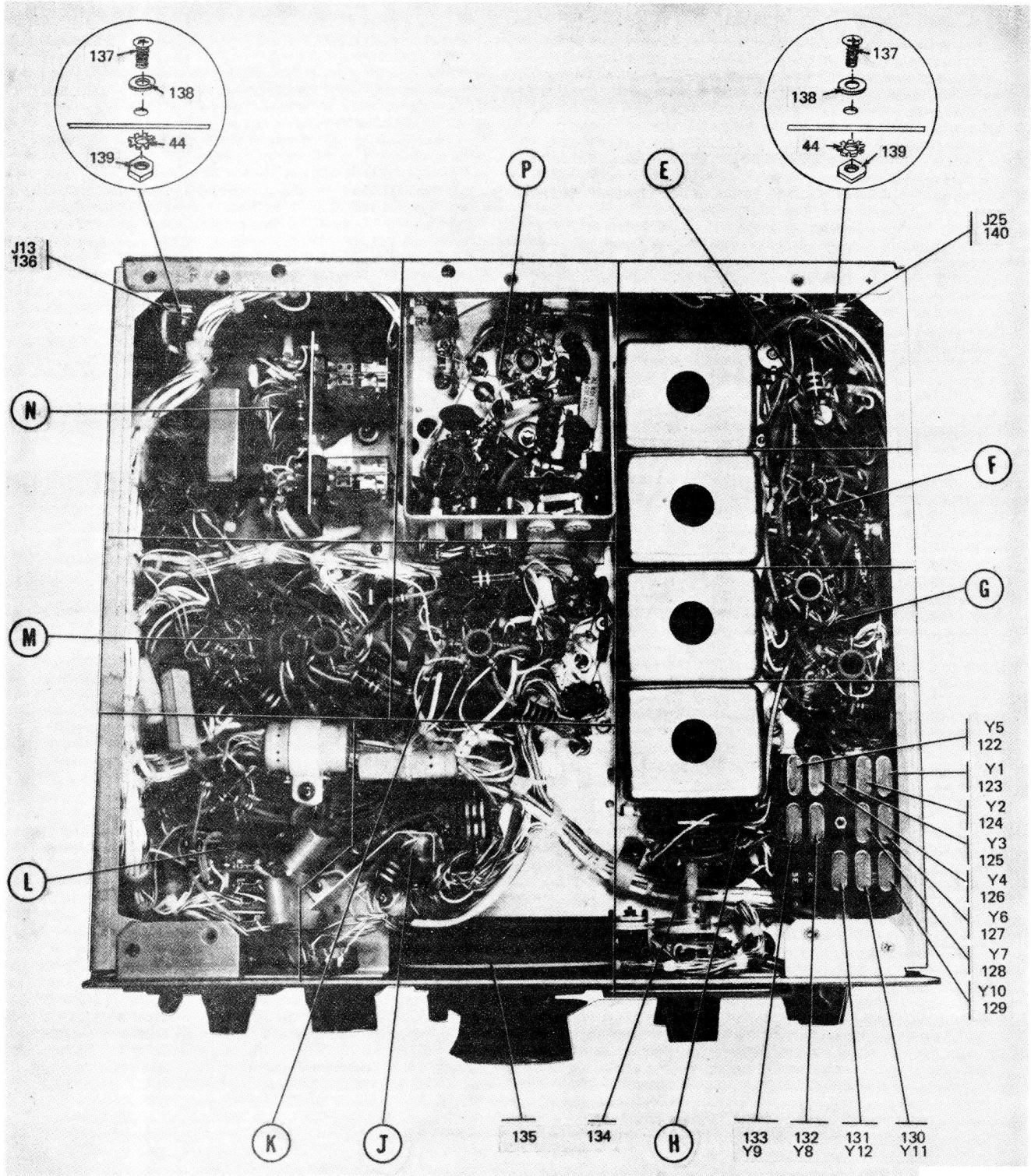
Figure 2 © Chassis subassembly (Sheet 6 of 20)
