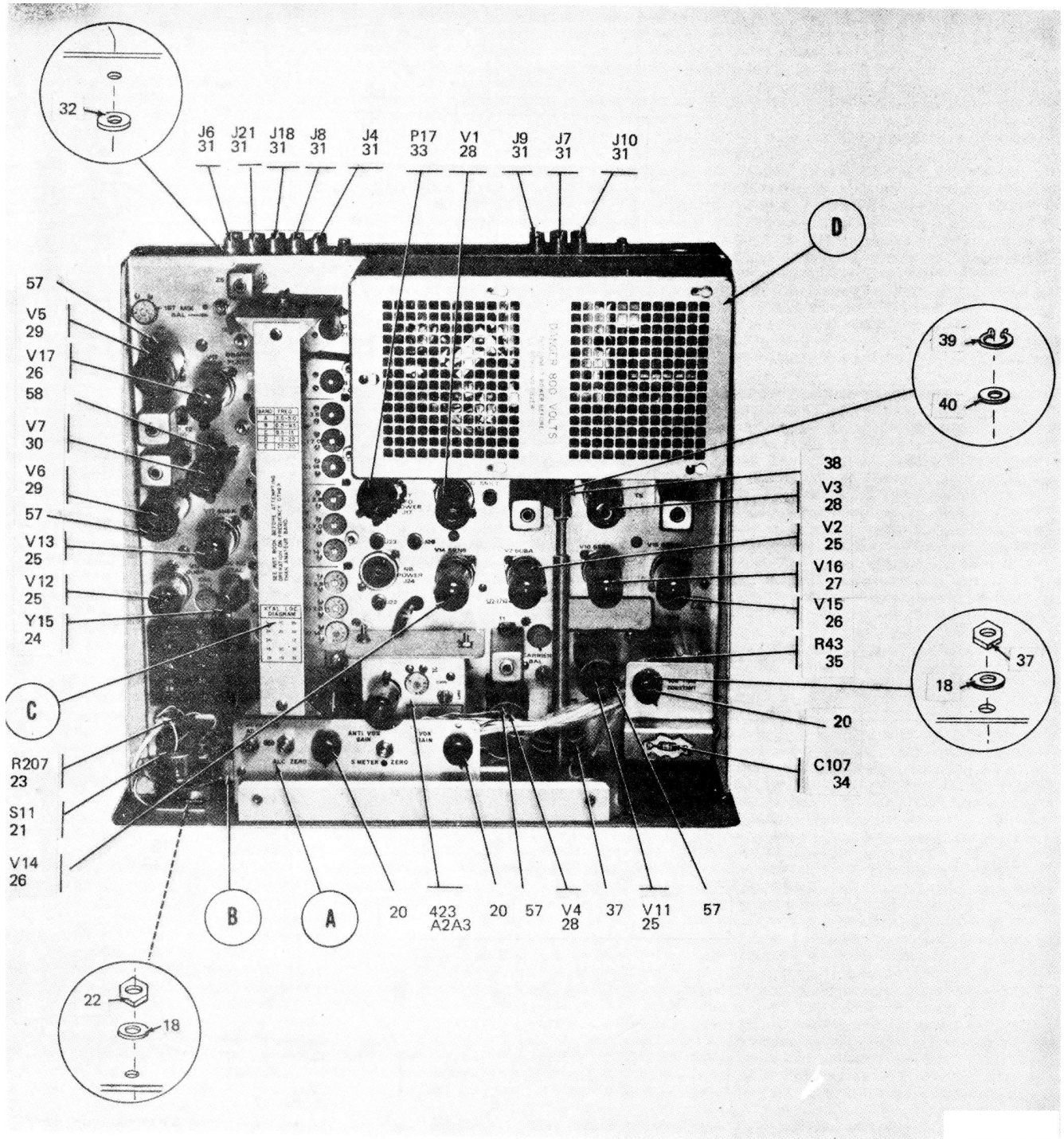
Figure 2. ② Chassis subassembly (Sheet 2 of 20).
