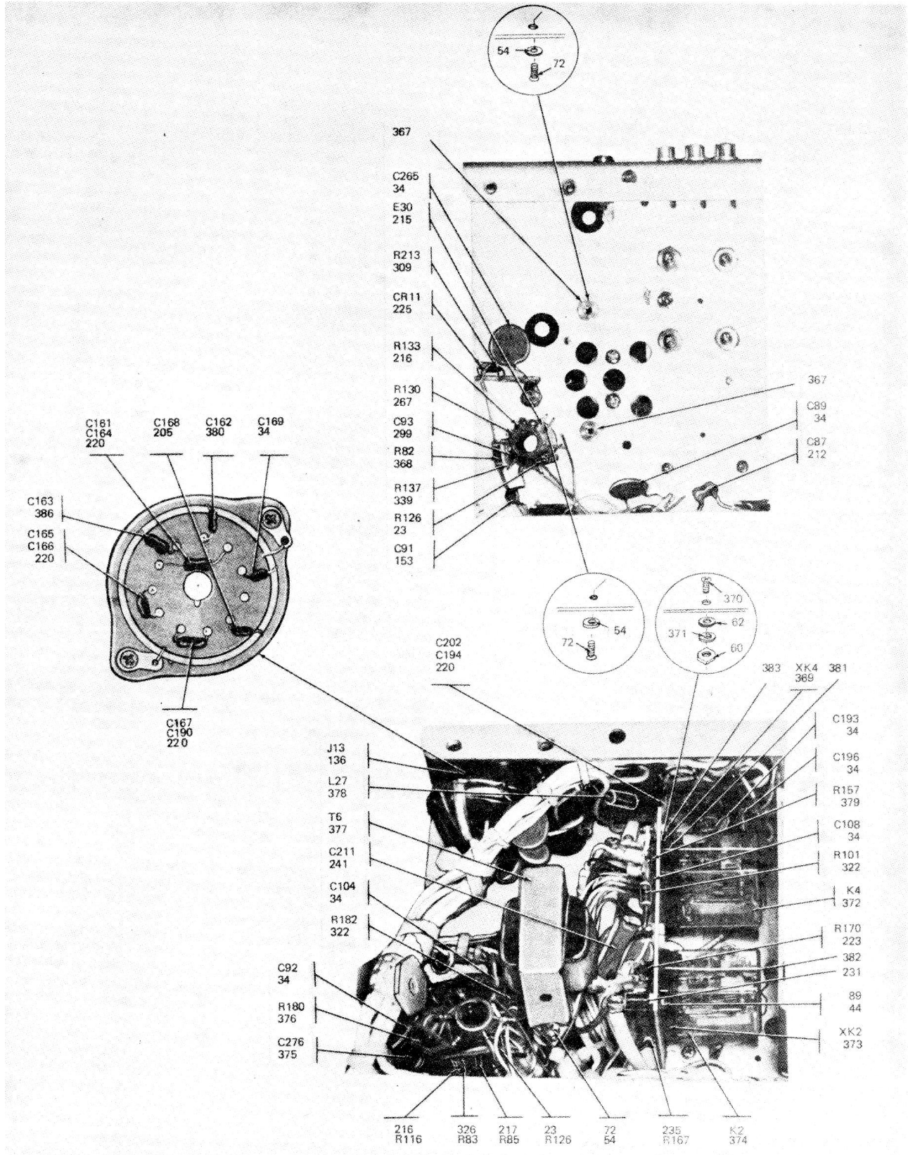
Figure 2. (18) Chassis subassembly (Sheet 18 of 20).
