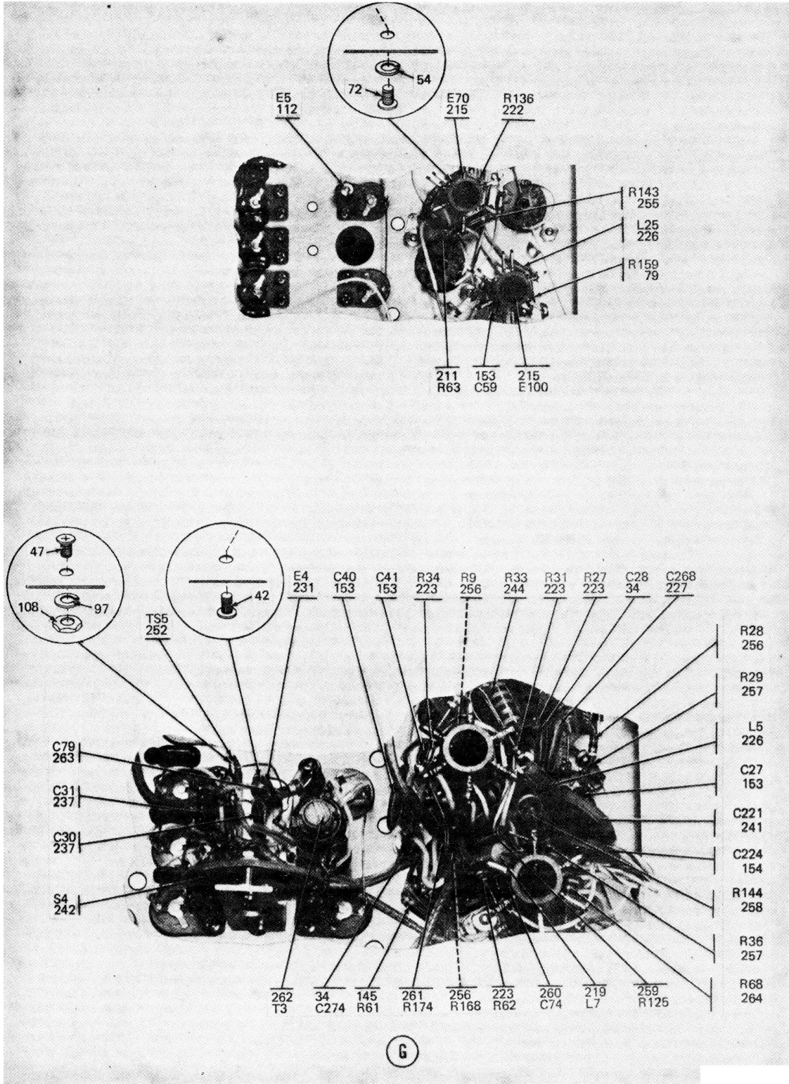
Figure 2. (12) Chassis subassembly (Sheet 12 of 20)
