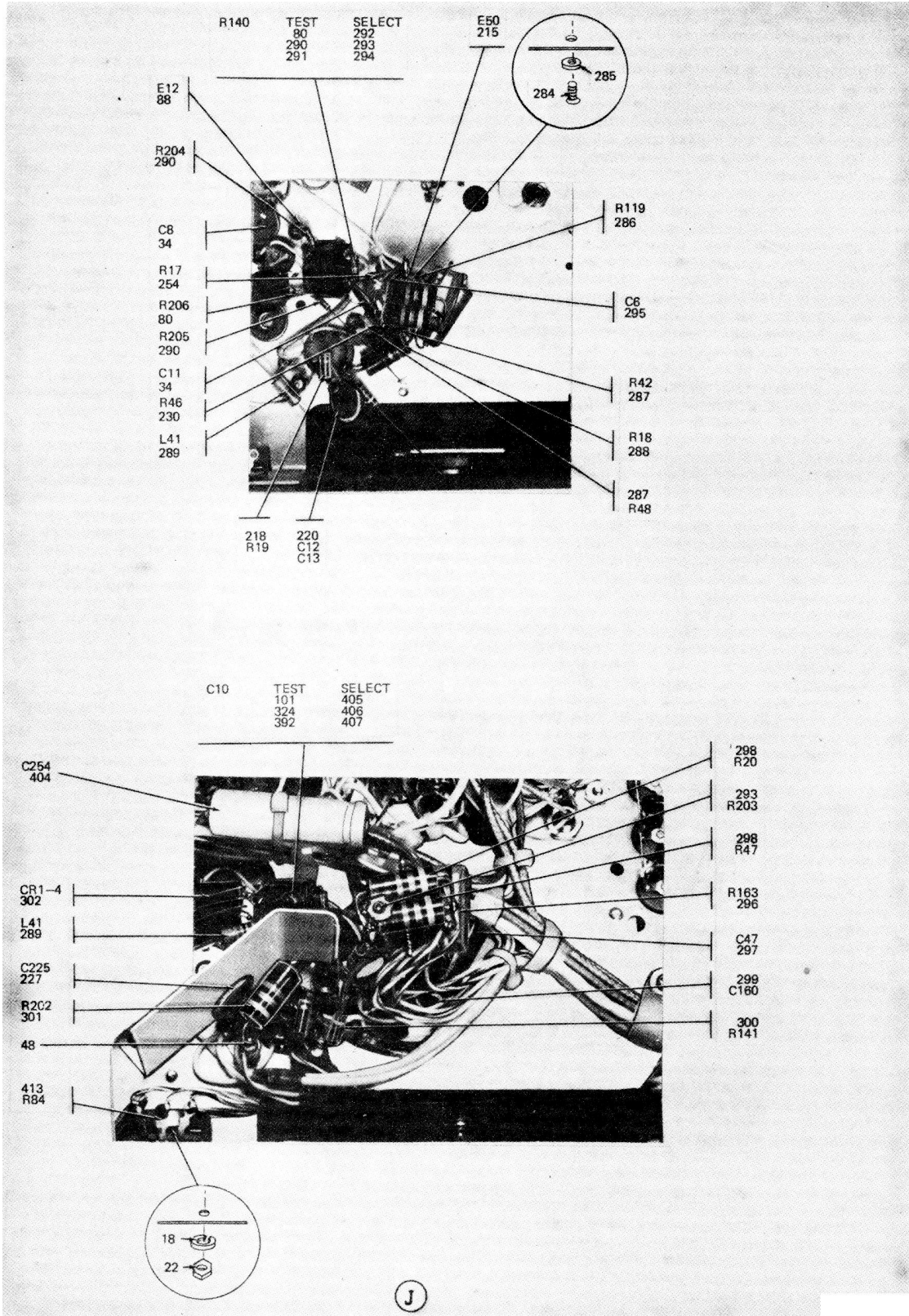
Figure 2. (14) Chassis subassembly (Sheet 14 of 20).
