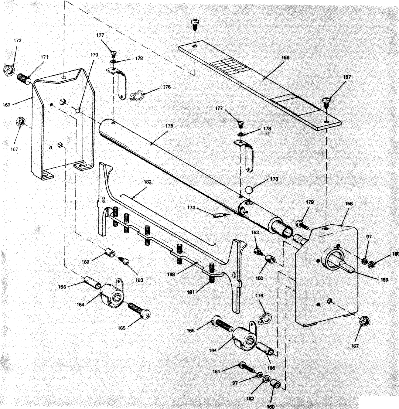
Figure 2 @ Chassis subassembly (Sheet 8 of 20).
