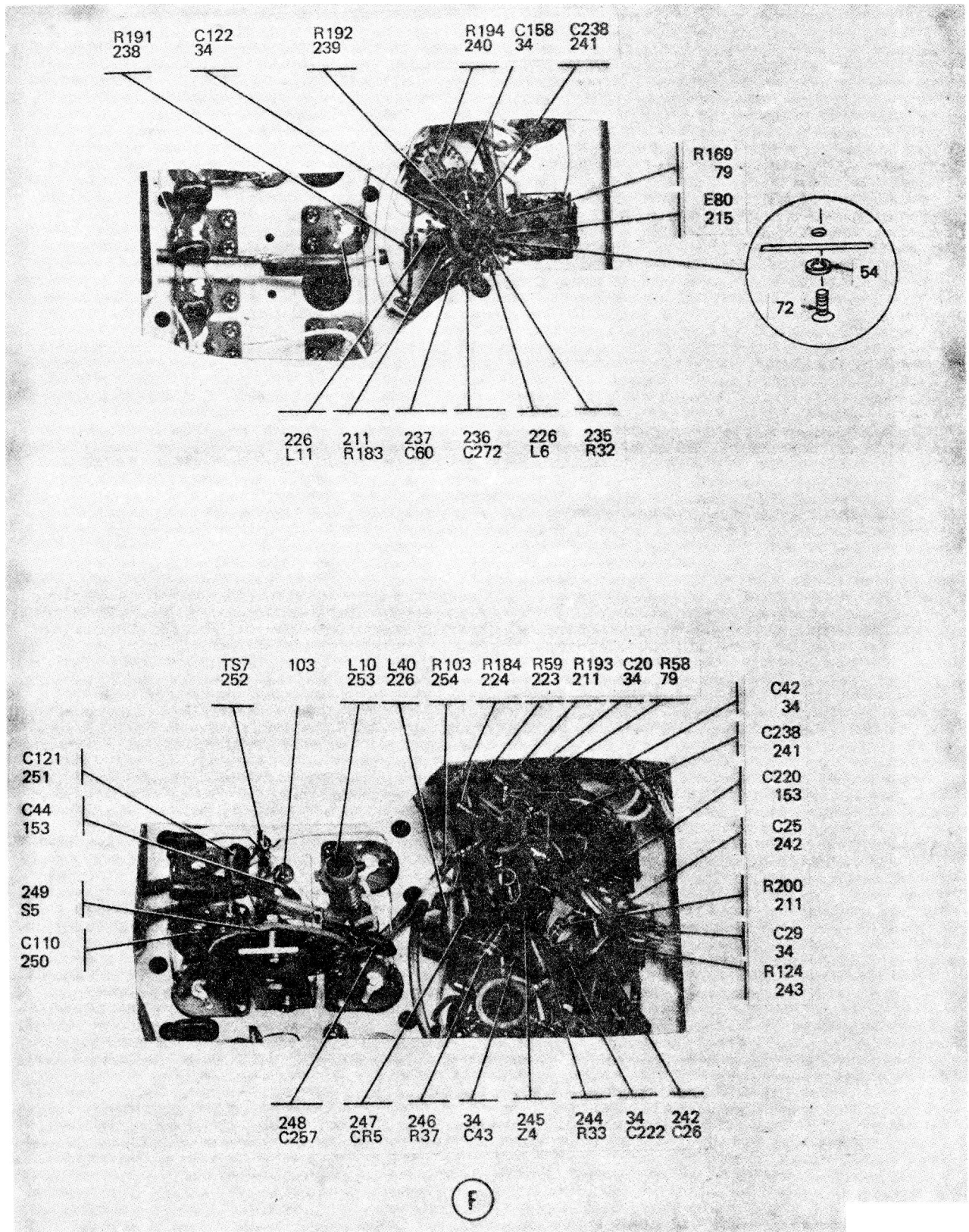
Figure 2. (1) Chassis subassembly (sheet 11 Of 20)
