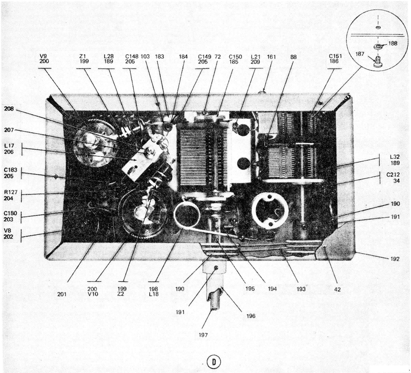
Figure 2Ⓣ Chassis subassembly (Sheet 9 of 20).
